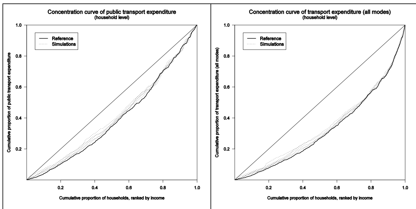
Figures 11 and 12: Concentration curves for public transport expenditure and total travel expenditure according to the observed distributions (thick line) and the simulated distributions (dotted lines) of household income
