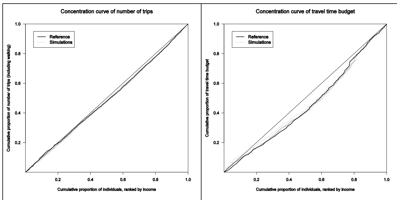
Figures 5 and 6: Concentration curves for total travel and travel time budget according to the observed distributions (thick line) and the simulated distributions (dotted lines) of individual income
