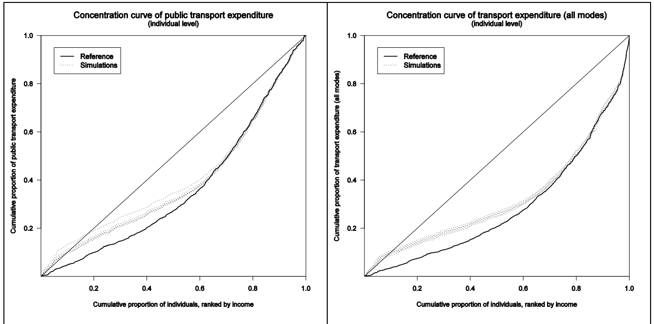
Figures 9 and 10: Concentration curves for public transport expenditure and total travel expenditure according to the observed distributions (thick line) and the simulated distributions (dotted lines) of individual income
