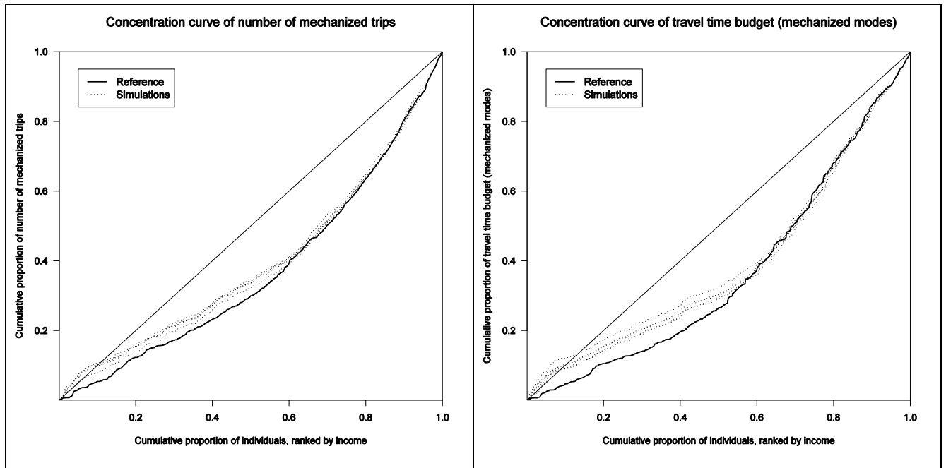
Figures 7 and 8: Concentration curves for mechanized mode travel and travel time budget according to the observed distributions (thick line) and the simulated distributions (dotted lines) of individual income
